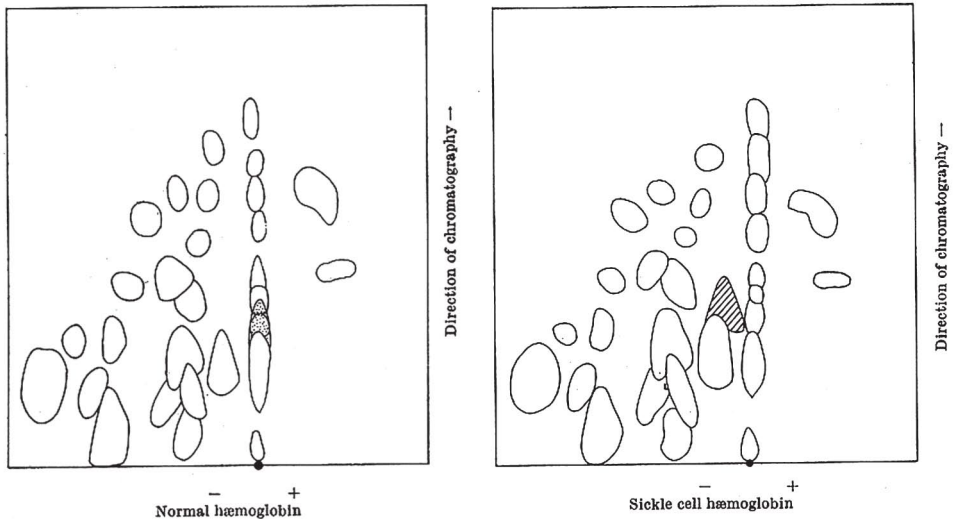
FIGURE 2.21. Vernon Ingram showed that the difference between normal hemoglobin (HbA) and sickle cell hemoglobin (HbS) was at the #6 position in the \beta -globin chain. ( Left ) Normal and ( right ) sickle cell hemoglobin fingerprints using electrophoresis.
