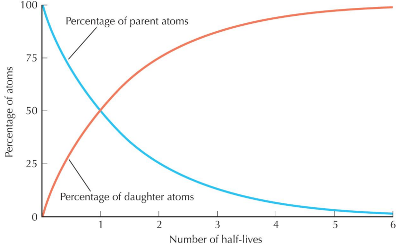
FIGURE 4.1. Radiometric dating. Graph showing the decline in the number of atoms of a radioactive isotope ( blue line ) and the increase in the number of atoms of daughter isotopes ( red line ).
