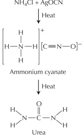
FIGURE 4.5. Synthesis of urea from inorganic salts by the Wöhler reaction.
