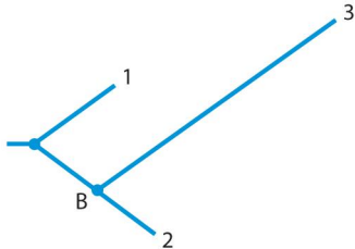
FIGURE 5.9. Unequal rates of evolution. A hypothetical phylogenetic tree showing relationships among three species. The rate of evolution of the lineage leading up to species 3 has accelerated relative to that of species 2, as indicated by the longer branch leading from their common ancestor (node B).
