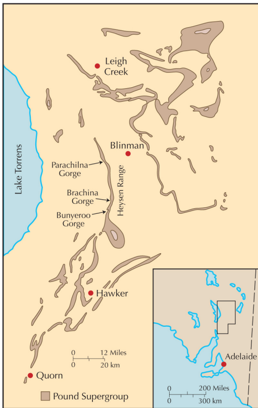
FIGURE 10.9. Location of the Ediacara site near Adelaide in southern Australia. The fossils occur in the Pound Supergroup, a major thickness of sedimentary rocks.
