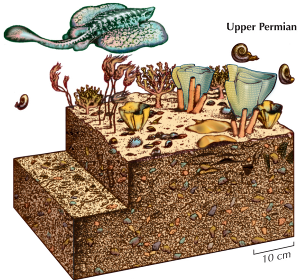
FIGURE 10.37. Effects of the Permian extinction. The latest Permian tropical seafloor compared with that of the Early Triassic, based on the section at Meishan, China, showing the loss of reef-dwelling organisms.
