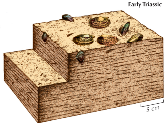
FIGURE 10.37. Effects of the Permian extinction. The latest Permian tropical seafloor compared with that of the Early Triassic, based on the section at Meishan, China, showing the loss of reef-dwelling organisms.
