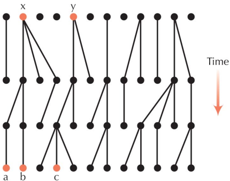
FIGURE 15.6. Identity by descent.
