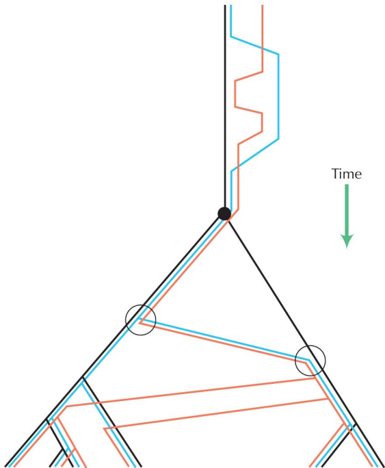
FIGURE 15.14. Coalescence with recombination.
