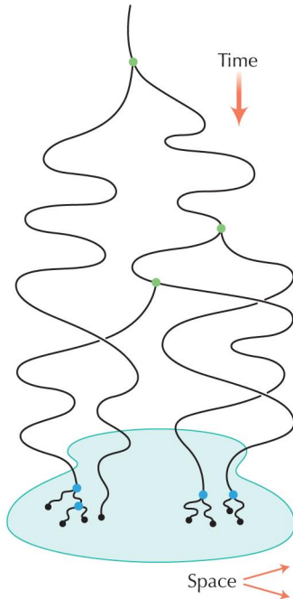
FIGURE 16.14. In a two-dimensional population, nearby genes may be closely related through a coalescence event in the recent past. Otherwise, lineages wander over a wide area as they trace back to a common ancestor in the distant past.
