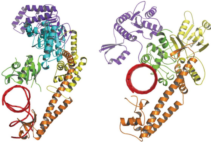
FIGURE 20.2. MutS ( left ) and topoisomerase II ( right ) bind DNA using very similar folds. However, the sequences of the proteins as a whole show that they are only distantly related. Colored regions show different domains.
