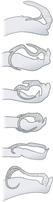
FIGURE 20.26. Male genitalia have evolved complex structures that aid competition with other males. Shown here are the penes of six species from the damselfly genus Argia . The stippled areas are used to scoop out sperm that have been stored by the female from previous matings.
