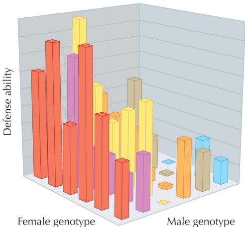
FIGURE 20.28. Genetic variation in sperm competition in Drosophila . The bars show the ability of a male's sperm to defend against displacement by a subsequent mating. This depends on an interaction between the genotypes of male and female. In this experiment, six male genotypes were tested against six female genotypes, giving 36 experiments in all.
