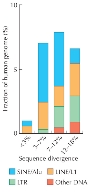
FIGURE 21.16. The distribution of ages of transposable elements in the human genome. This is measured by divergence from the human–mouse consensus sequence and is grouped into bins that correspond to about 25 Myr of divergence.
