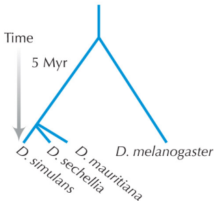
FIGURE 22.9. This phylogeny shows the relationships between flies in the Drosophila melanogaster species group, which will be discussed throughout this chapter.
