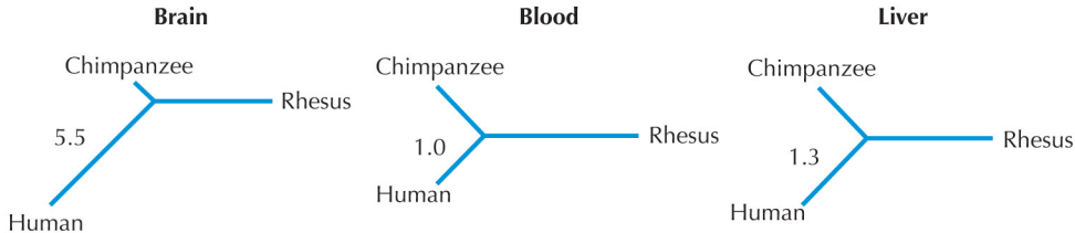
FIGURE 25.26. The relative extent of changes in gene expression among three primate species and three tissues. Numbers give the extent of change in the lineages leading to humans relative to those leading to chimpanzees.
